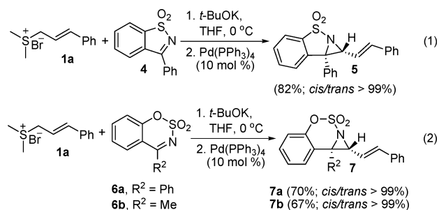
Scheme 1. Aziridination of Cyclic Imines 4 , 6a , and 6b
